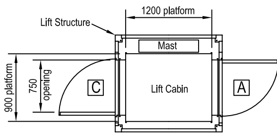
Landing Door Entrance Positions
