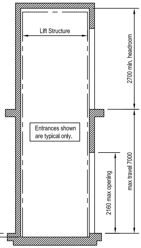
Lift Shaft Detail (optional)
