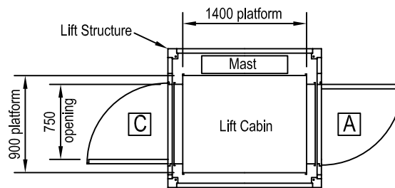
Landing Door Entrance Positions
